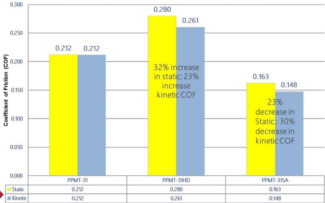
COF comparison of PropylMatte 31, 31HD and 31SA
